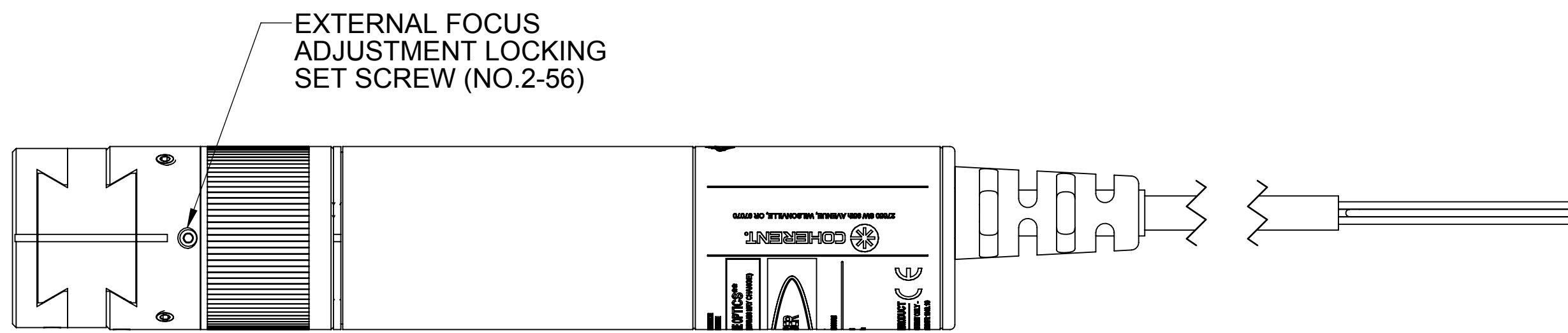
TOP VIEW
