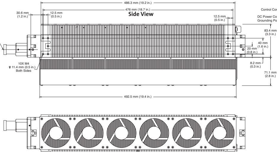
Bottom View
